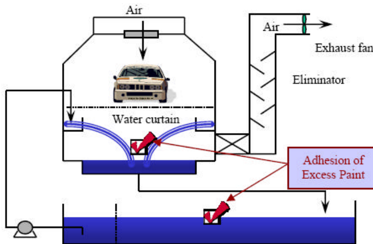
TYPICAL PAINT BOOTH SYSTEM
